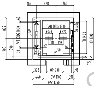
Hoistway plan/1:60
