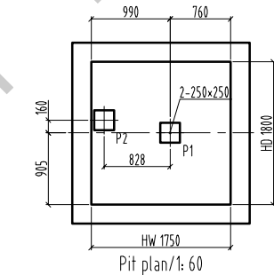
Pit plan/1: 60
