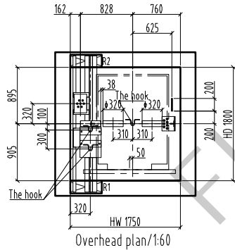
Overhead plan/1:60
