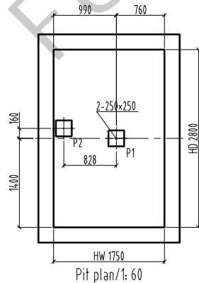
Pit plan/1: 60
