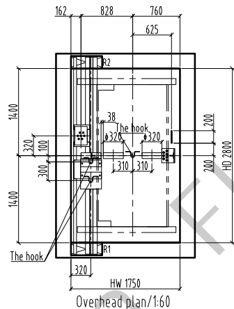
Overhead plan/1:60
