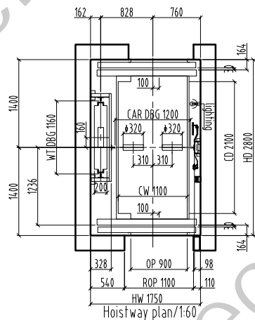
Hoistway plan/1:60
