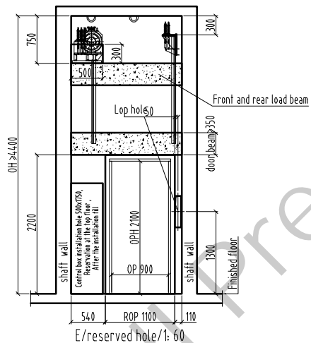
E/reserved hole/1: 60
