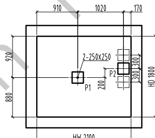
Pit plan/1: 60
