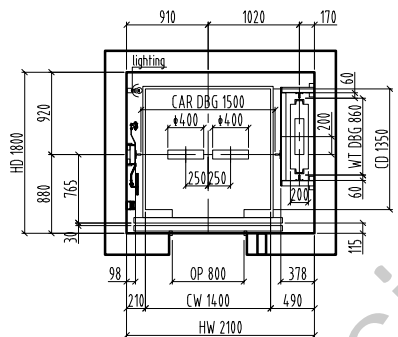
Hoistway plan/1:60
