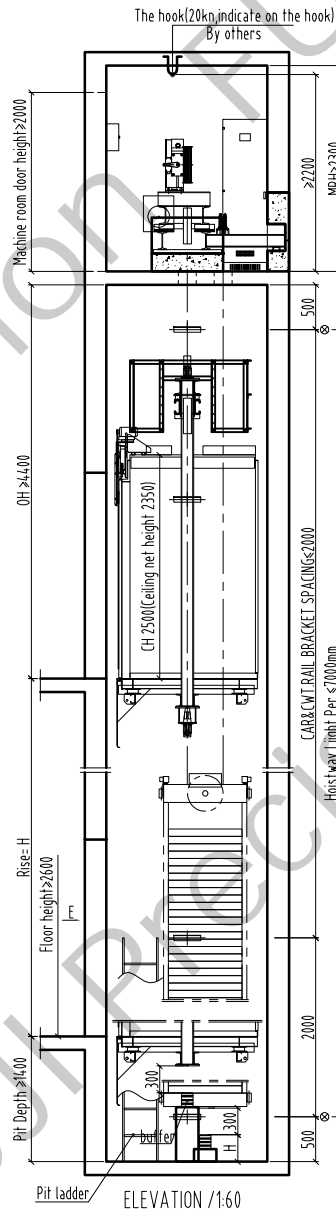
ELEVATION /1:60
