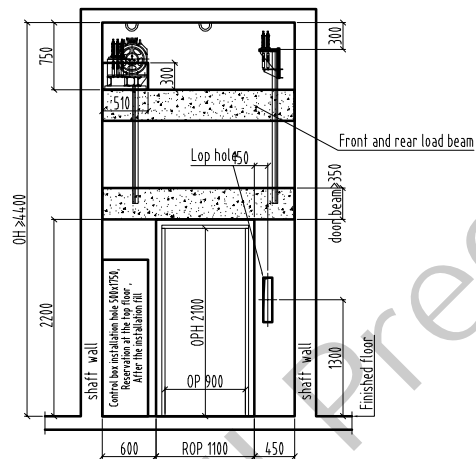
E/reserved hole/1: 60
