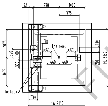
Overhead plan/1:60
