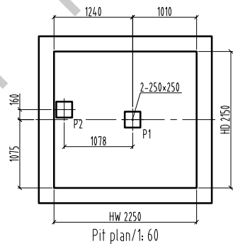
Pit plan/1: 60
