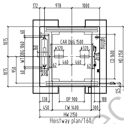
Hoistway plan/1:60
